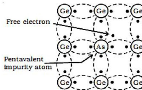
Figure: Lattice structure extrinsic
