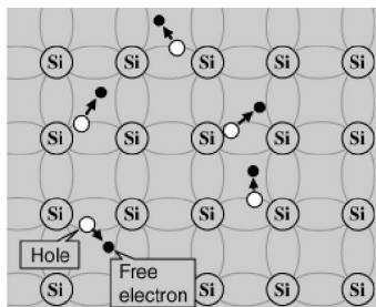
Figure: Lattice structure for intrinsic
